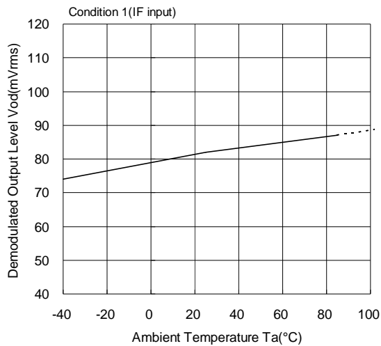
Demodulated Output Level versus Temperature
